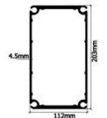
Main Frame Profile
