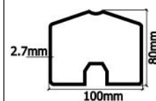
Eave Purlin
